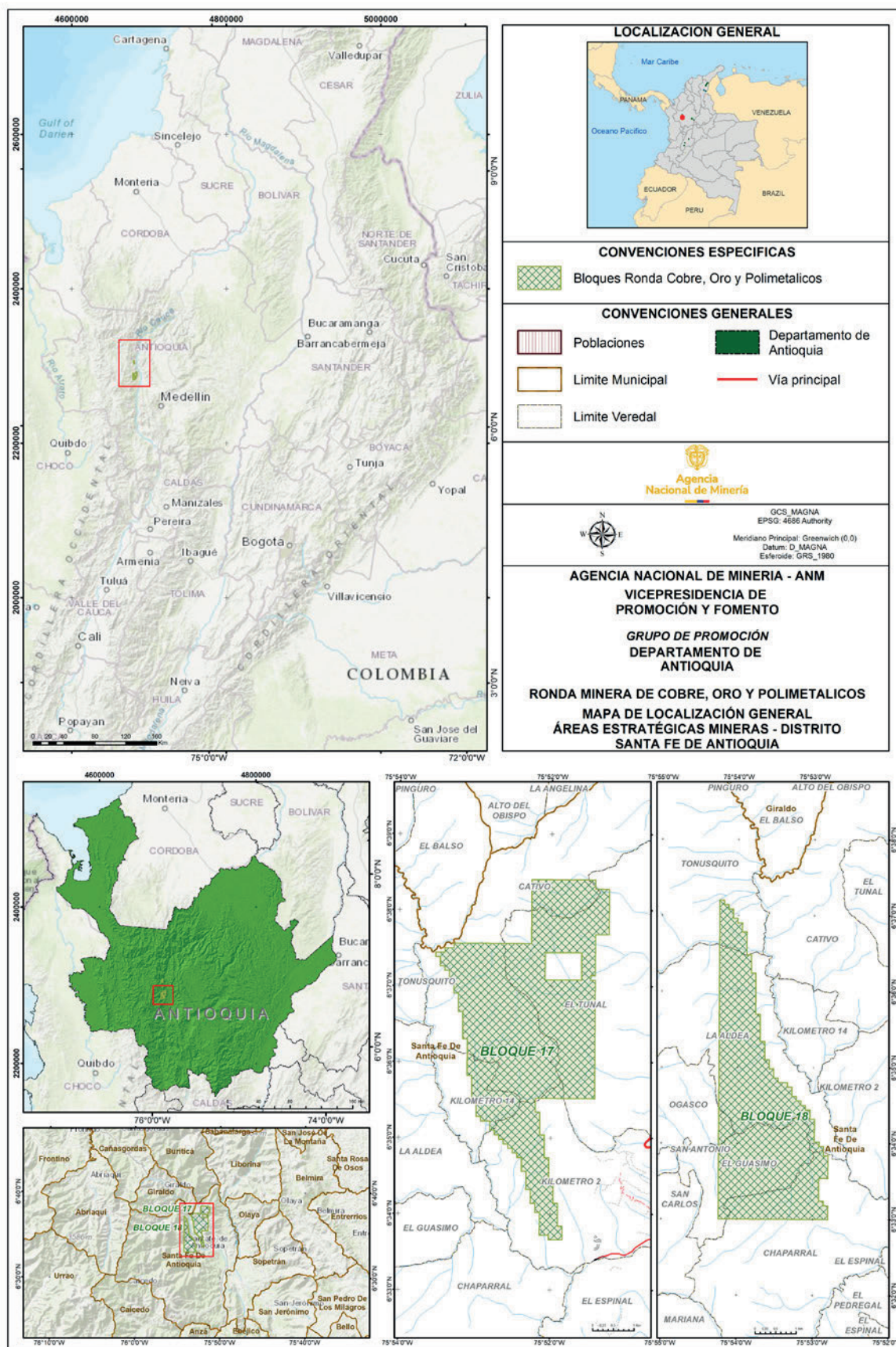
Figure 10: Regional geology and AEM Buriticá block diagram
