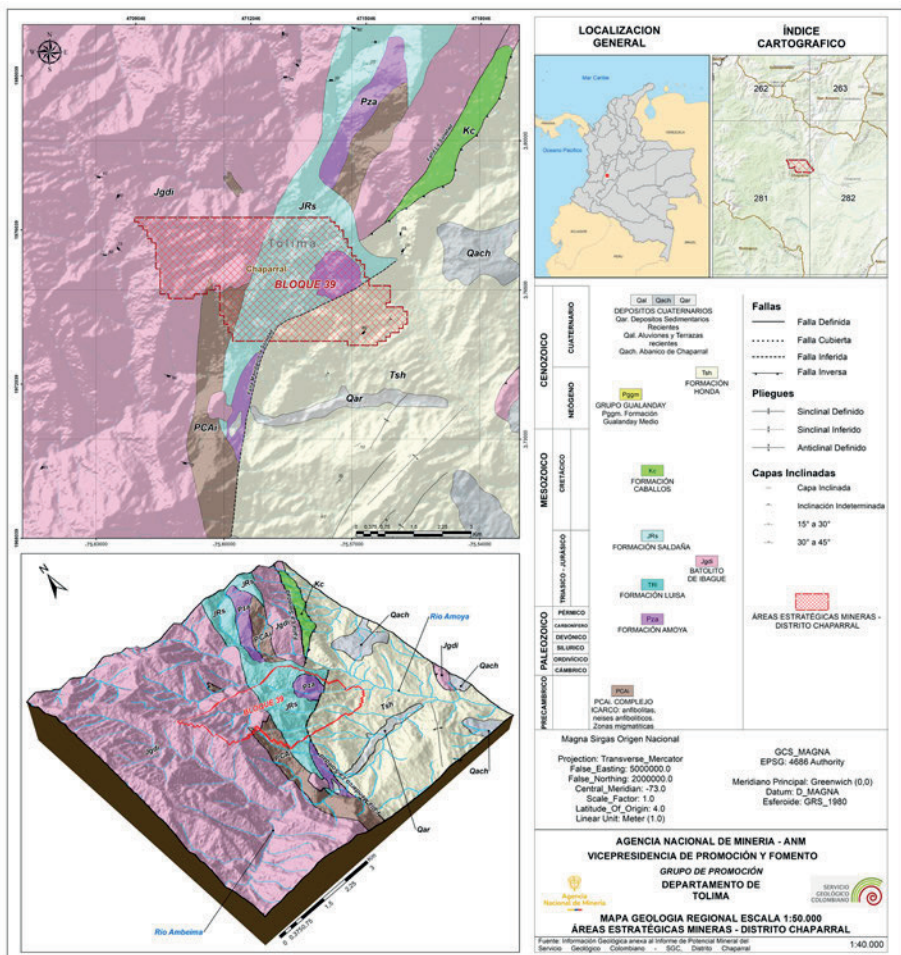
Figure 24: Regional geology and block diagram – Chaparral
